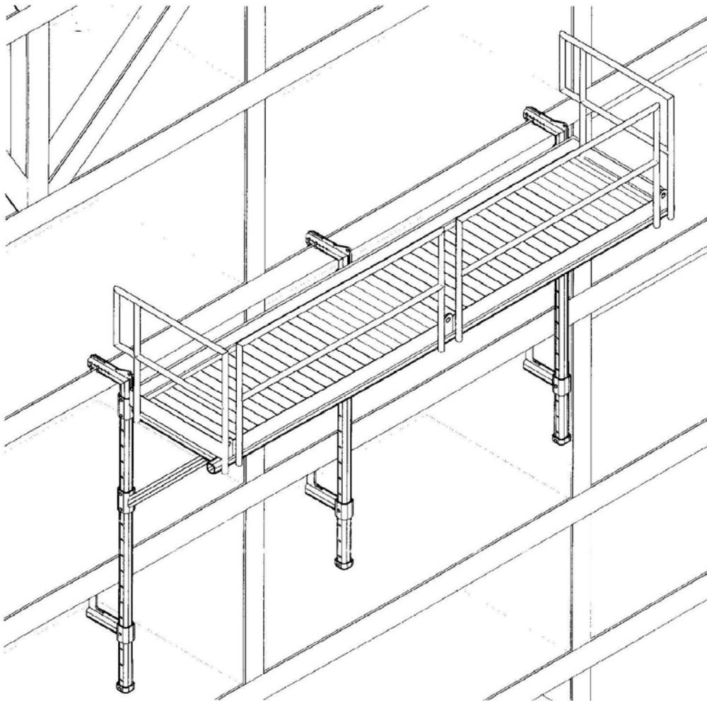
FIGURE 22-1 Hanging Scaffold
