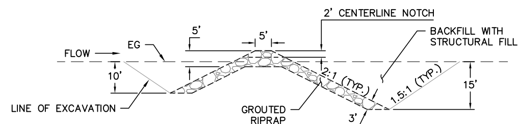
GRADE CONTROL STRUCTURE DETAIL NTS
